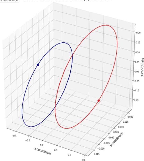
Visualization of orbits of stars in a two-body system from COM
