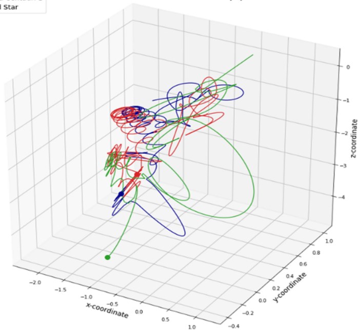
Visualization of orbits of stars in a two-body system
