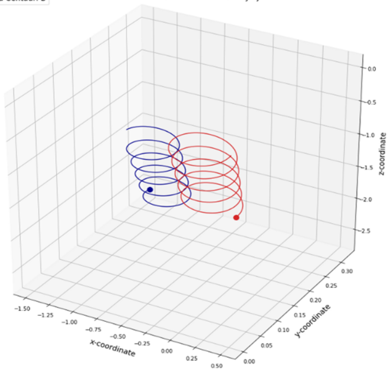
Visualization of orbits of stars in a two-body system
